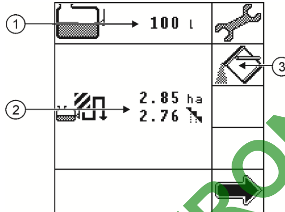
"Tank Control II" menu for one tank
